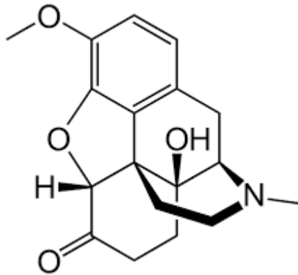
Oxycodonmolekyl
